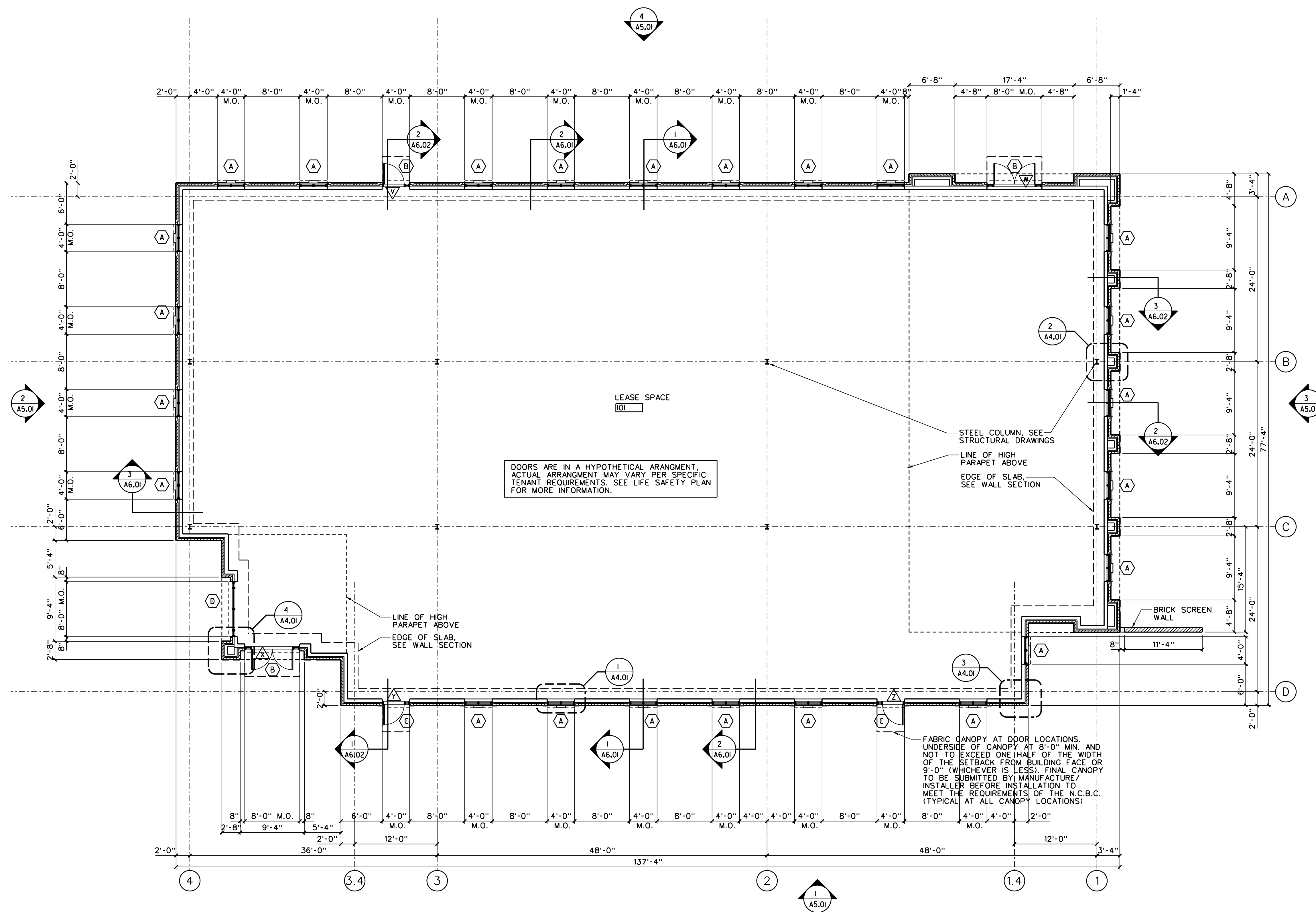
1 FLOOR PLAN 1/8" = 1' - 0"
